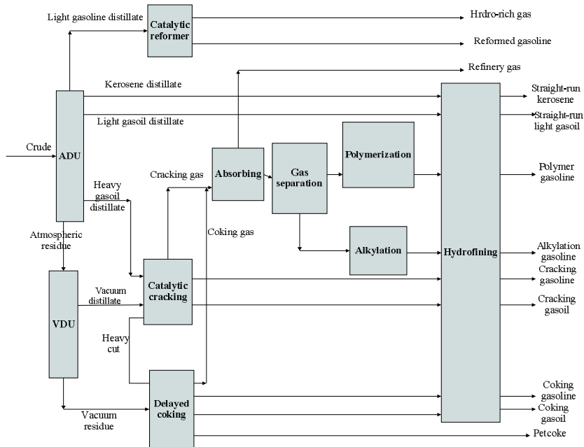
Chart: Processing Flow of Fuel Refineries
